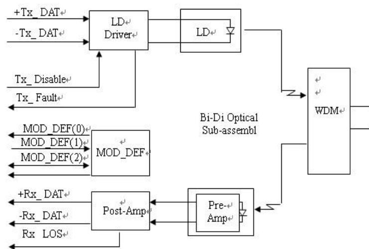
Block Diagram
